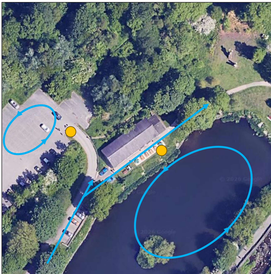
Figure 3.5: Bat Activity – 09/07/2026
